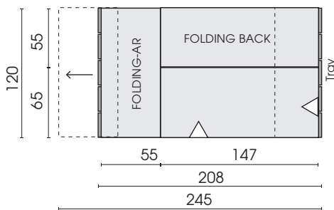
Sofa 2,5-seat armrest left with motorised seat adjustment 98M
