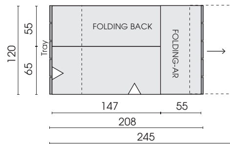
Sofa 2,5-seat armrest right with motorised seat adjustment 97M
