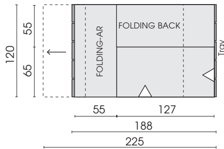
Sofa 2-seat armrest left with motorised seat adjustment 26M
