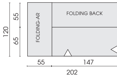
Sofa 2,5-seat armrest left 258
