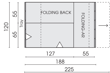
Sofa 2-seat armrest right with motorised seat adjustment 25M
