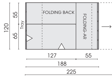
Sofa 2-seat armrest right with manual seat adjustment 225
