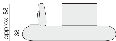
Front view (type 824 / 2 x type 609A)
