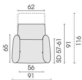
Functional amchair, swivel & rocking system 2 AR 100F
