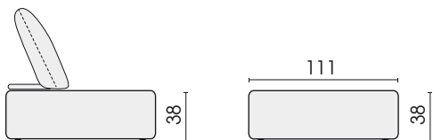
Side view seat element, deep (with back type 611)
