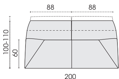
Sofa 2,5-seat, 2 AR 240
