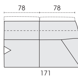
Sofa 2-seat, AR right 210
