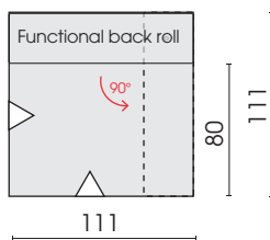
Element functional back, right 11T
