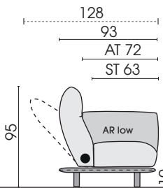
Side view 240FH
