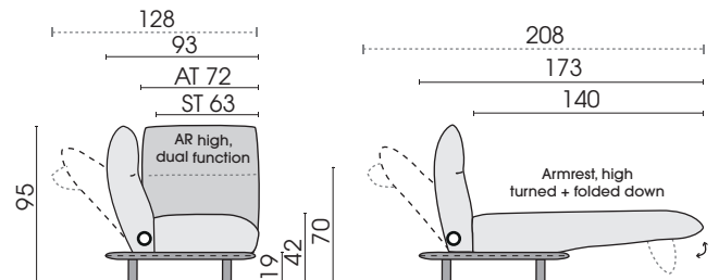
Side view M240DFH
