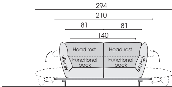
Front view 240DFH / M240DFH
