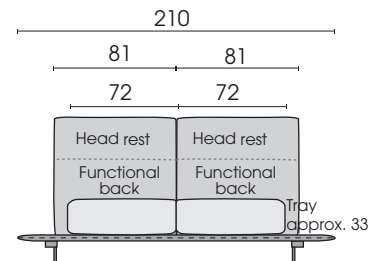
Front view 240FH / M240FH, turned into a lounger
