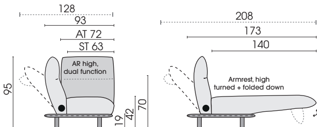
Side view 240DFH
