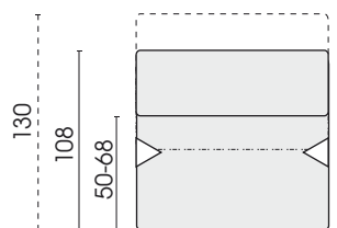
Element, back motorised M130
